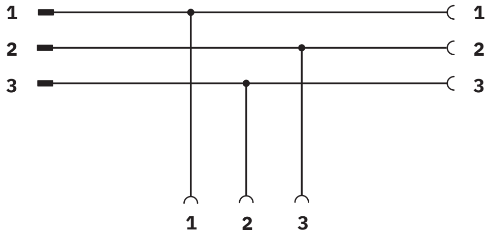
Circuit diagram
