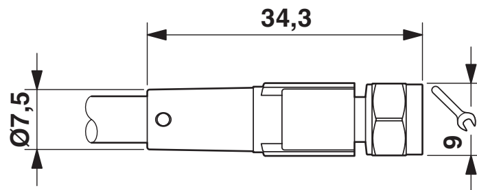
Dimensional drawing
