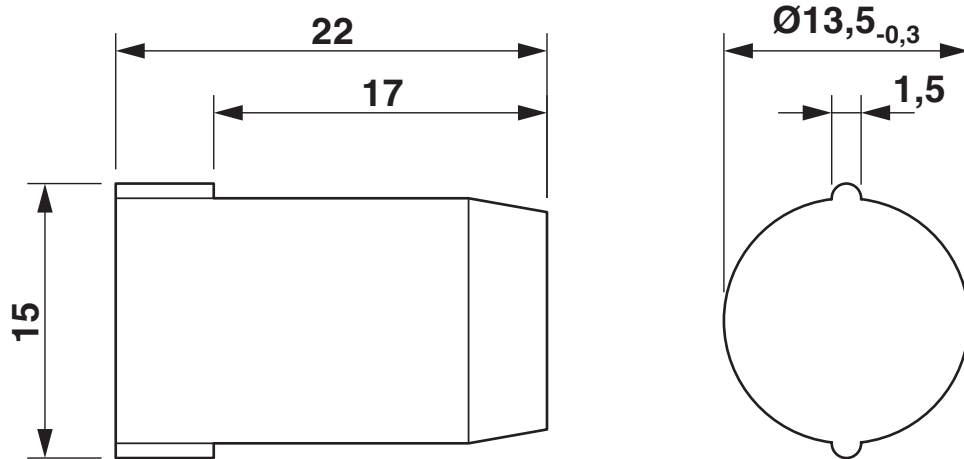
Dimensional drawing
