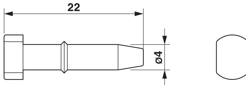
Dimensional drawing
