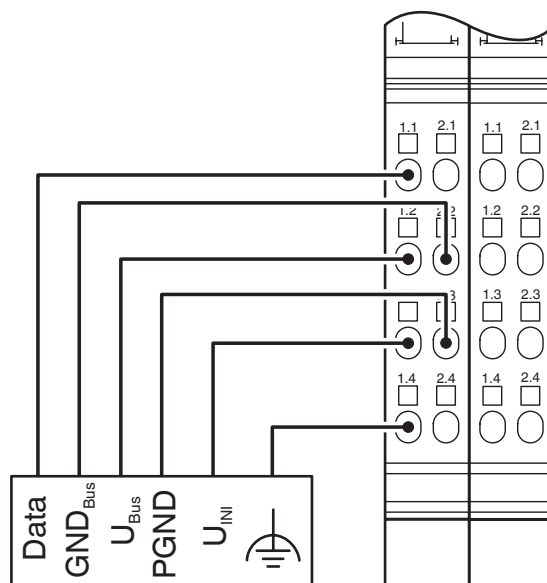
Connection diagram
