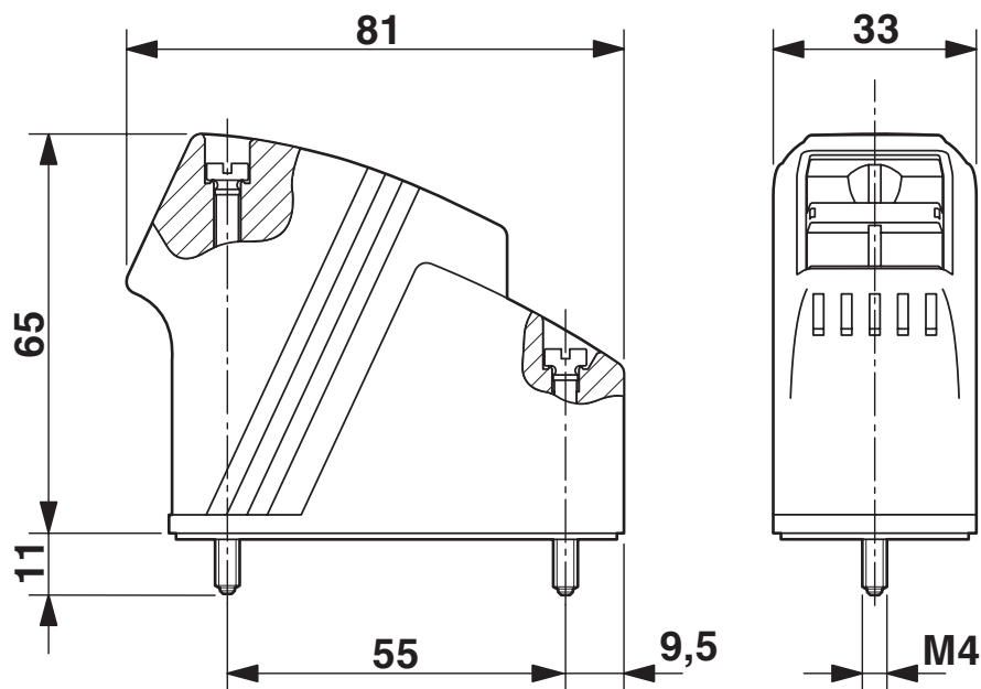
Dimensional drawing
