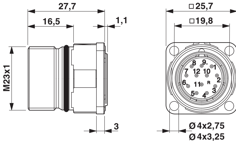
Dimensional drawing
