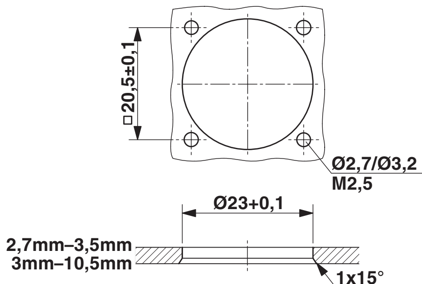
Dimensional drawing
