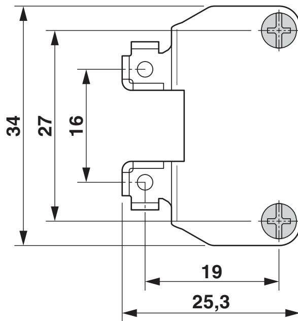
Dimensional drawing
