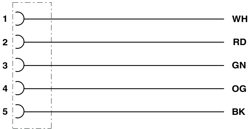
Contact assignment of 7/8" socket
