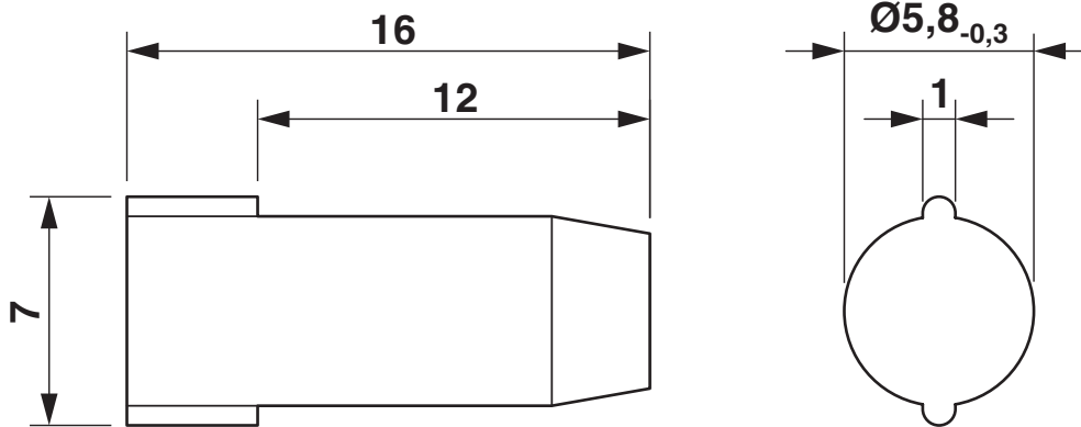
Dimensional drawing
