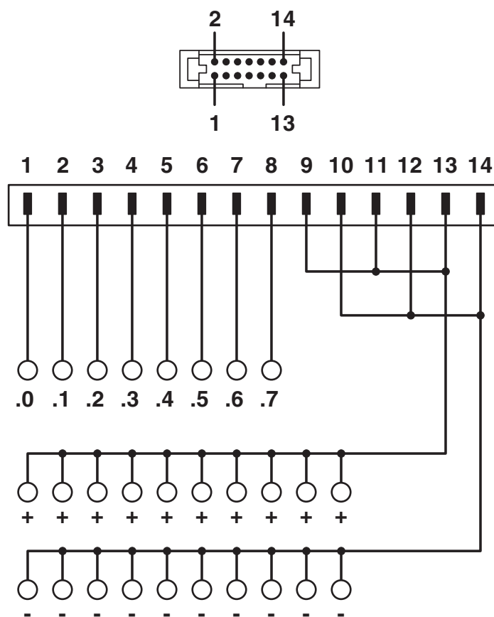
Circuit diagram
