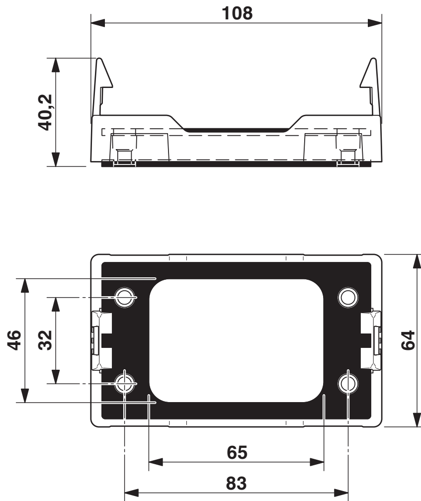
Dimensional drawing
