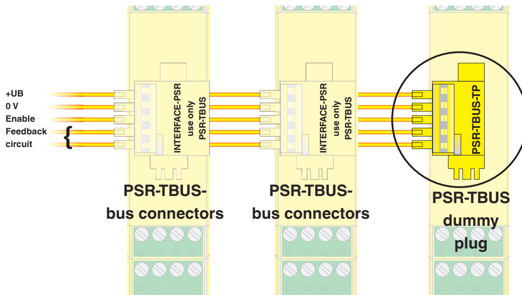
Connection diagram
