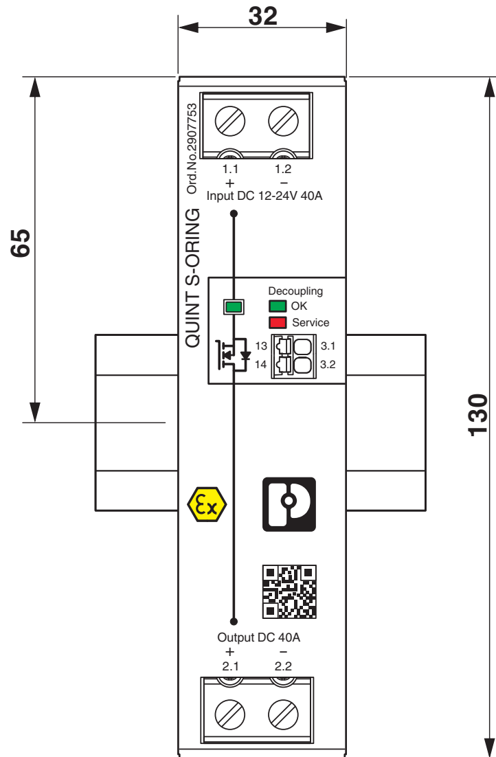
Dimensional drawing
