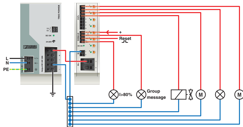
Application drawing
