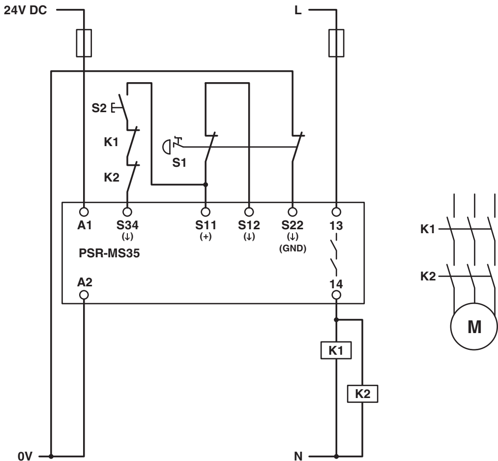
Application drawing
