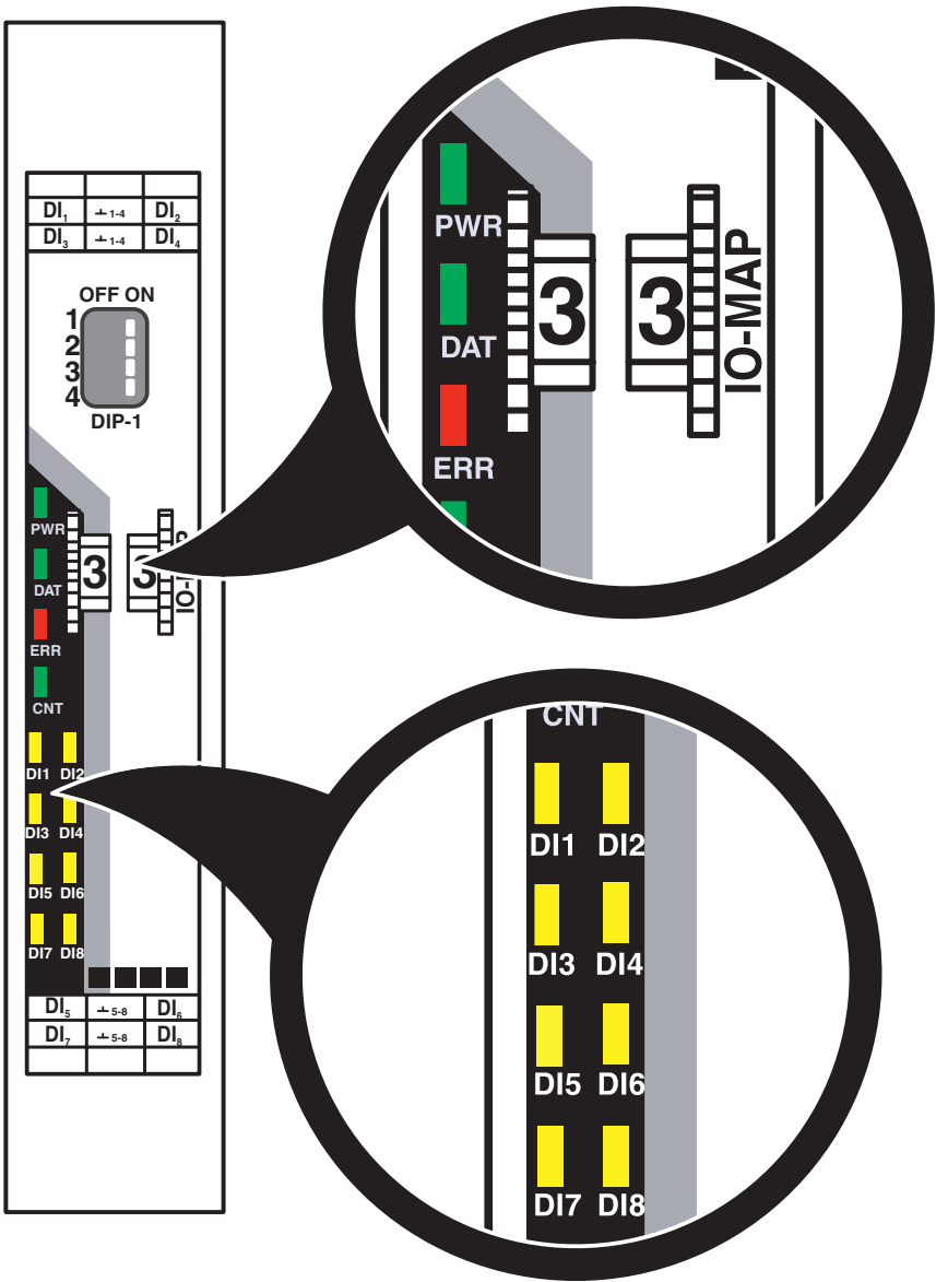
Schematic diagram
