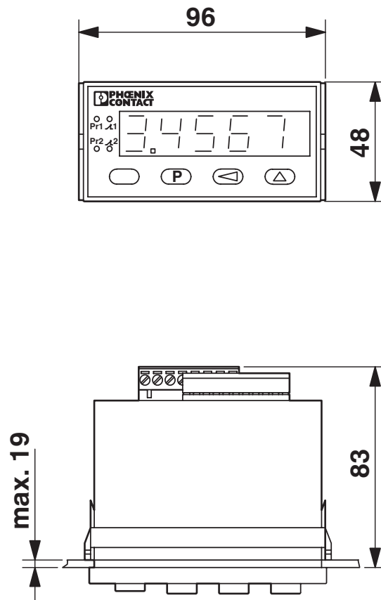
Dimensional drawing
