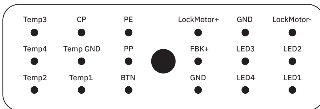
Connection diagram
