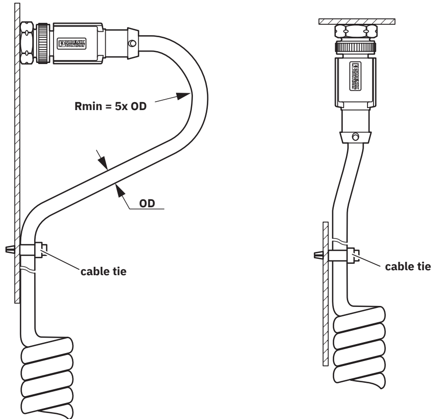
Application drawing
