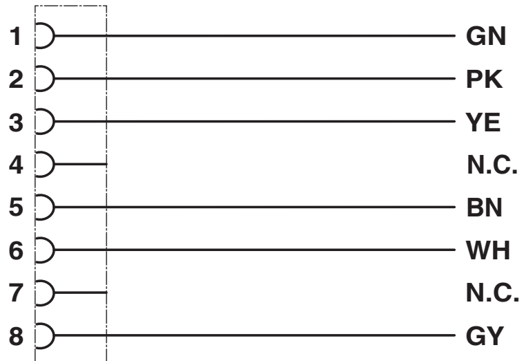
Circuit diagram
