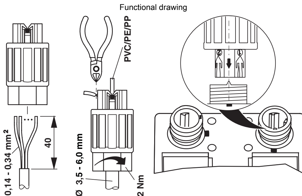
Schematic diagram
