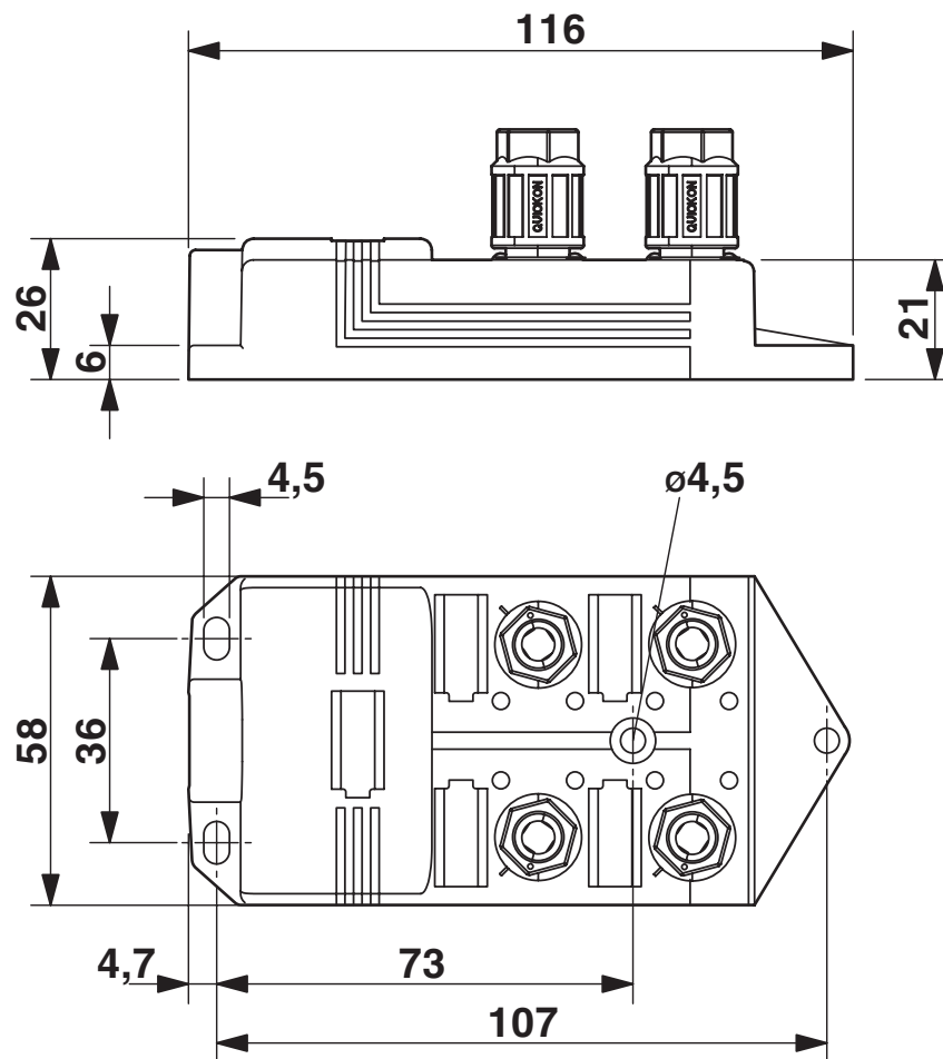
Dimensional drawing
