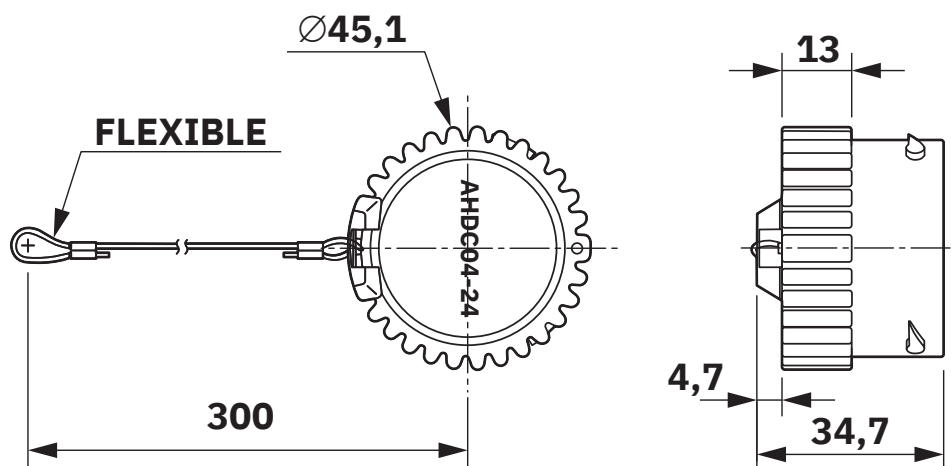
Dimensional drawing
