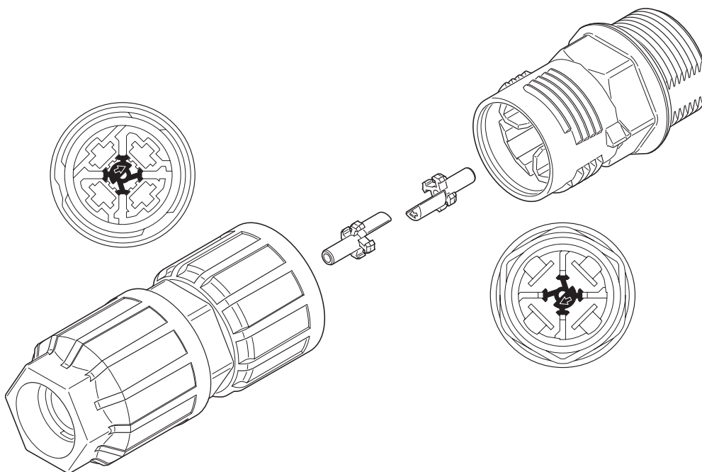
Schematic diagram
