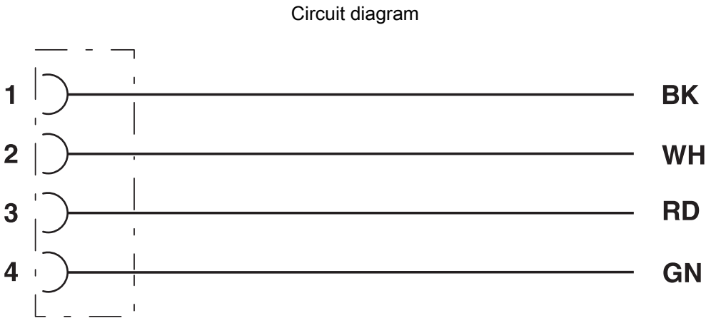
Contact assignment of 7/8" socket
