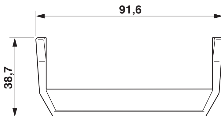
Dimensional drawing
