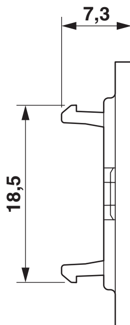
Dimensional drawing
