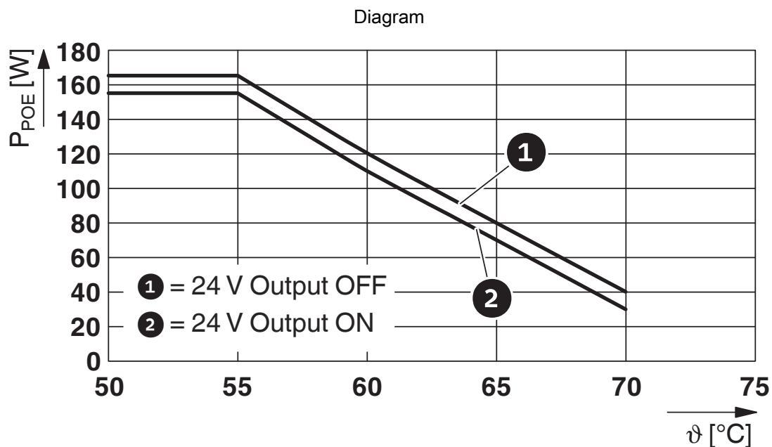
Derating (PoE power total)
