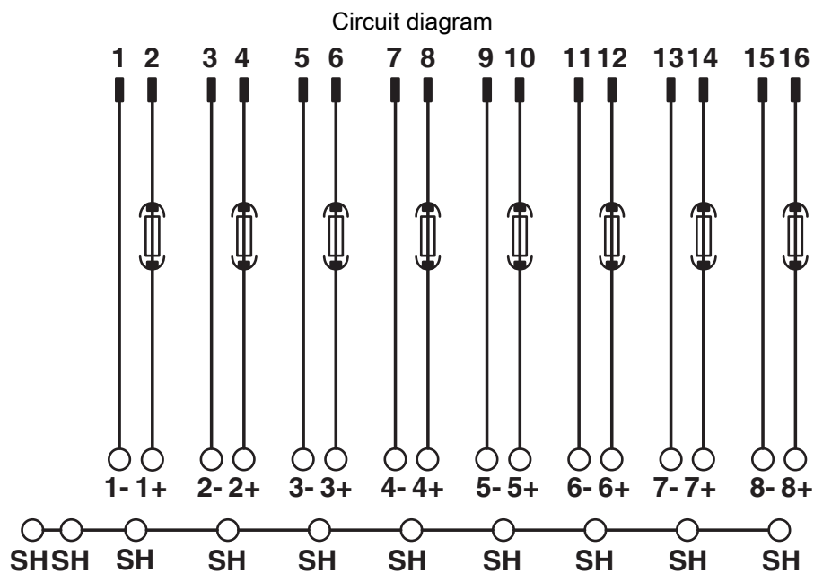
Connection scheme UM-DELTAV/D/SI
