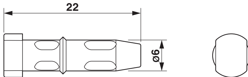
Dimensional drawing
