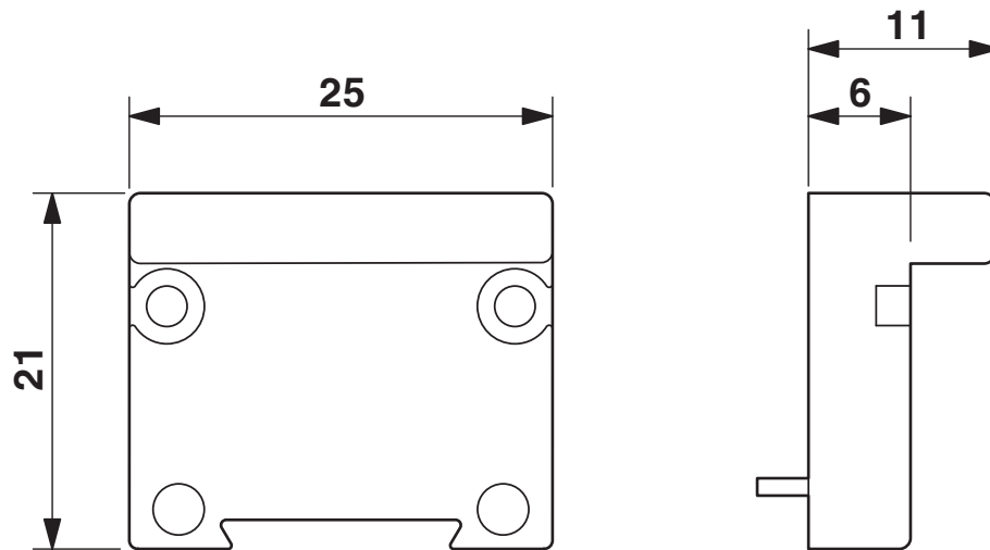
Dimensional drawing
