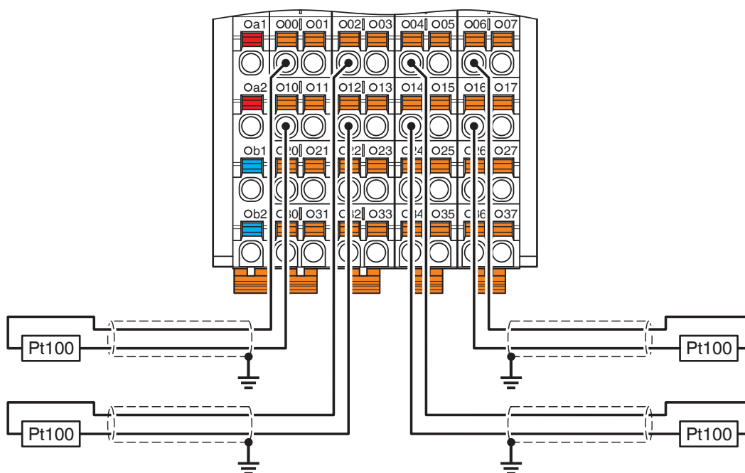
Connection diagram
