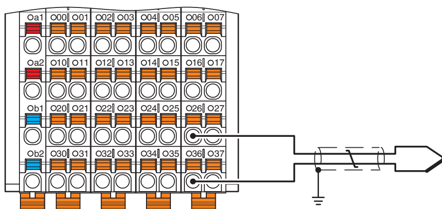
Connection diagram
