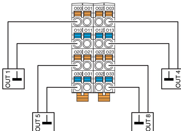
Connection diagram
