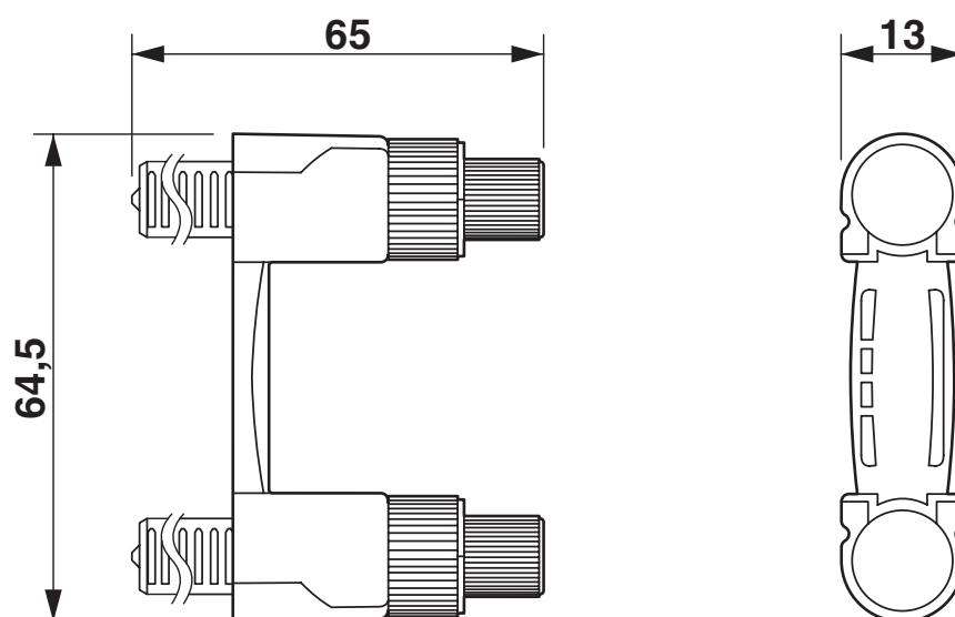
Dimensional drawing
