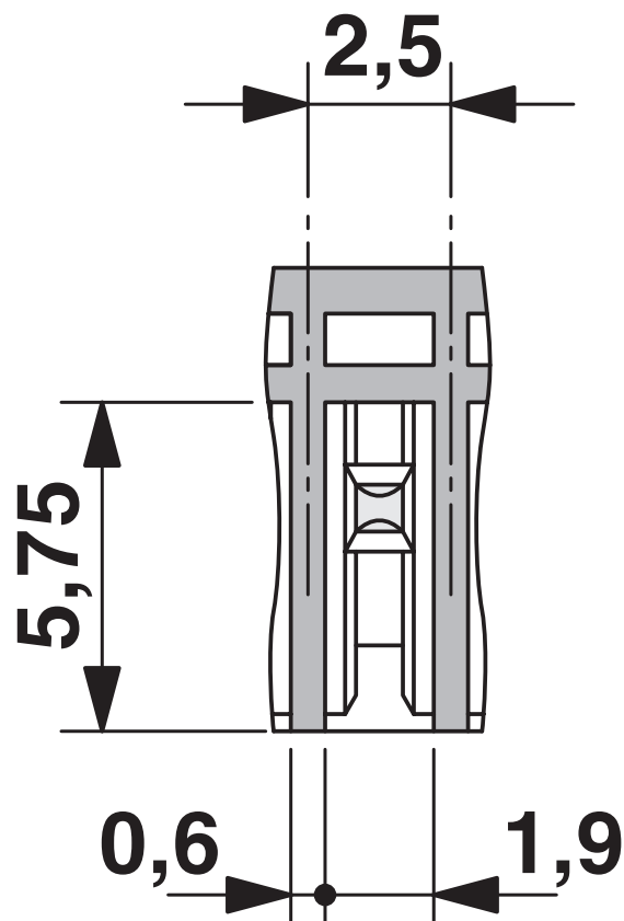
Dimensional drawing
