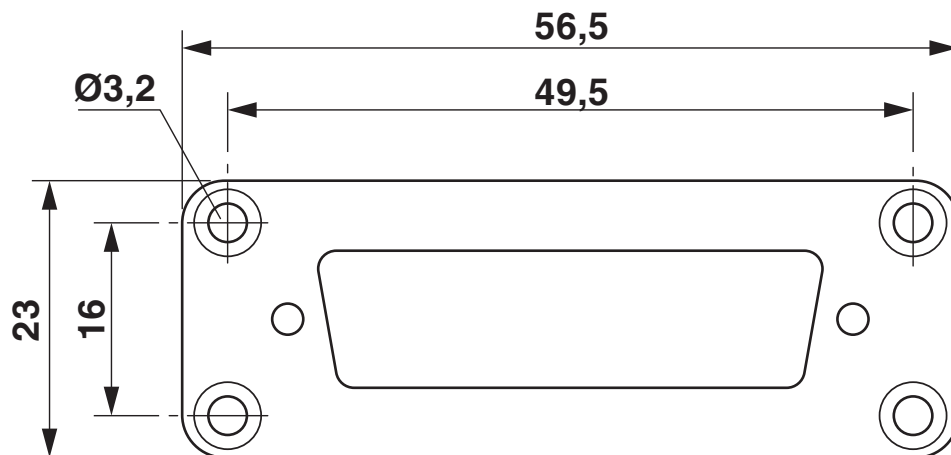
Dimensional drawing
