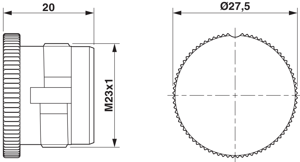
Dimensional drawing
