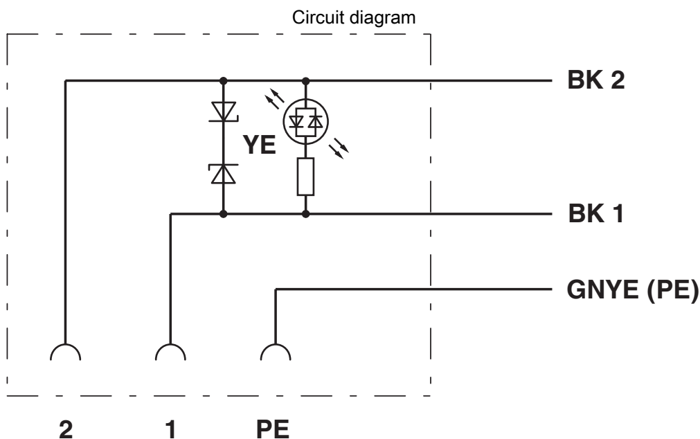
Contact assignment of the valve plug
