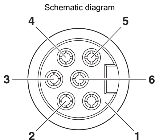
Circuit diagram
