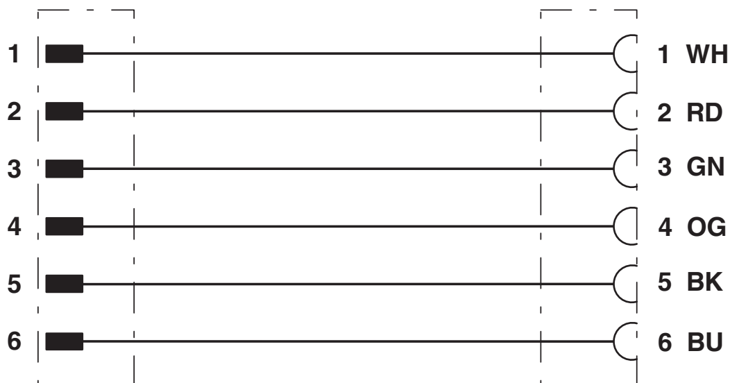
Circuit diagram
