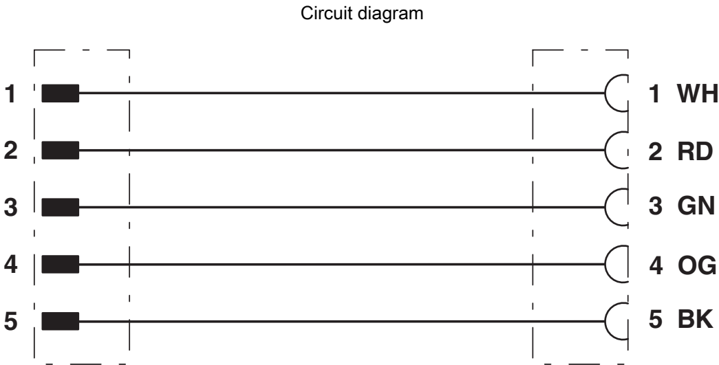
Contact assignment of 7/8" plug
