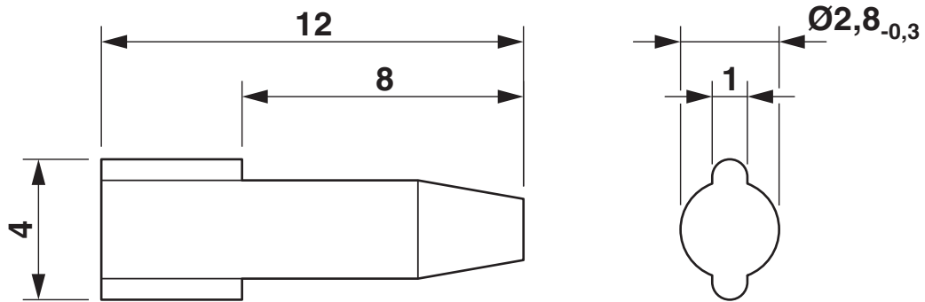
Dimensional drawing
