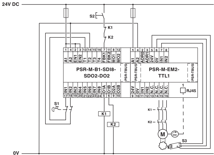
Application drawing
