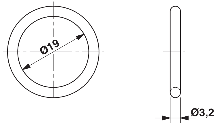
Dimensional drawing
