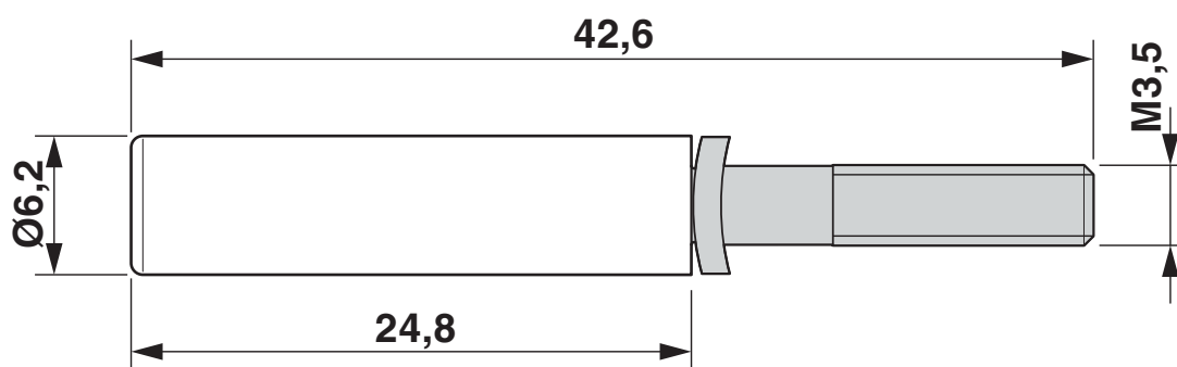
Dimensional drawing
