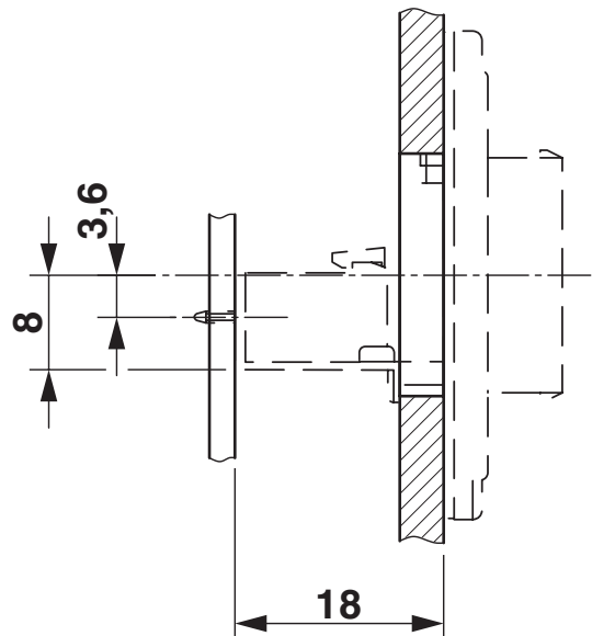
Dimensional drawing
