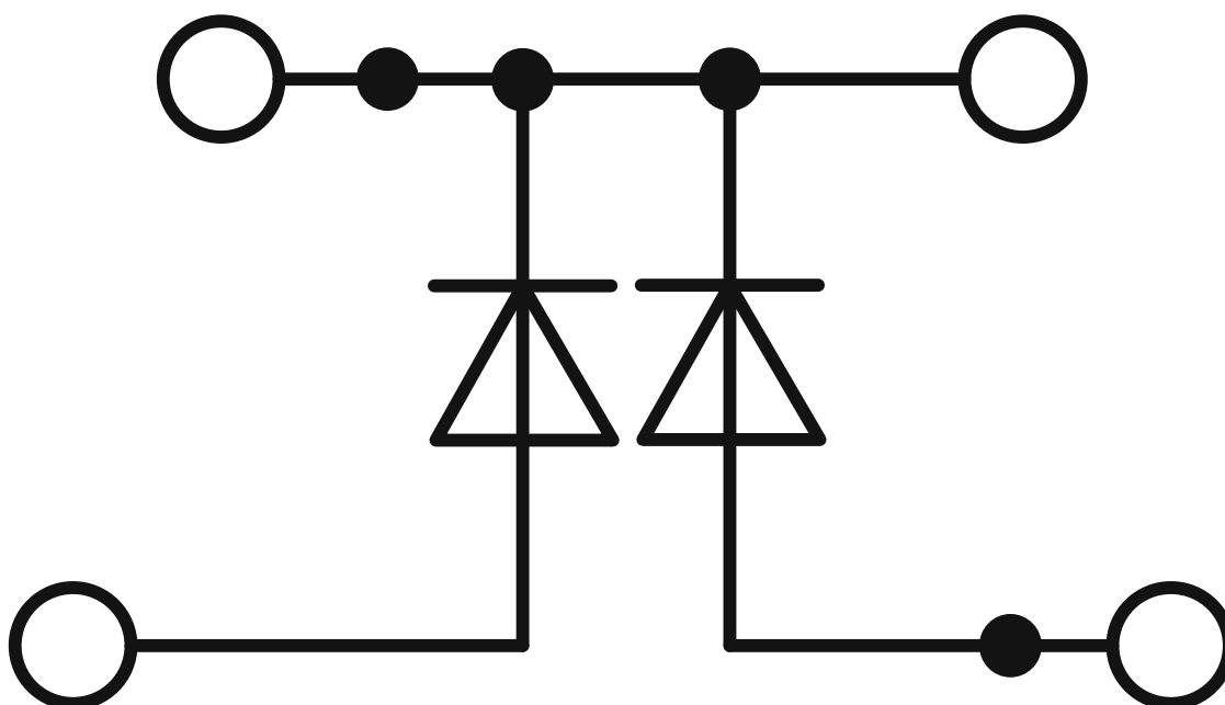
Circuit diagram
