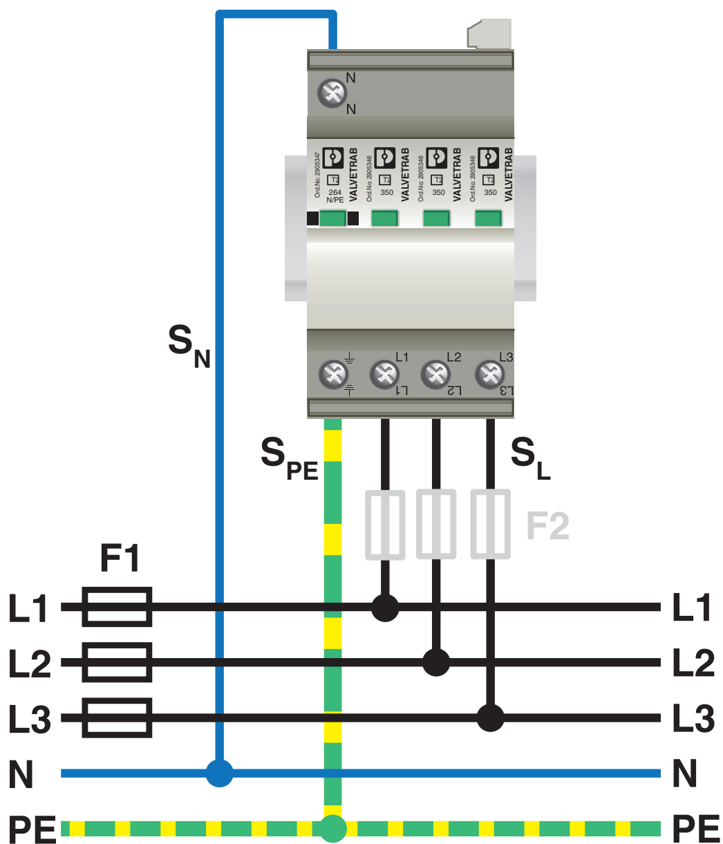
Application drawing
