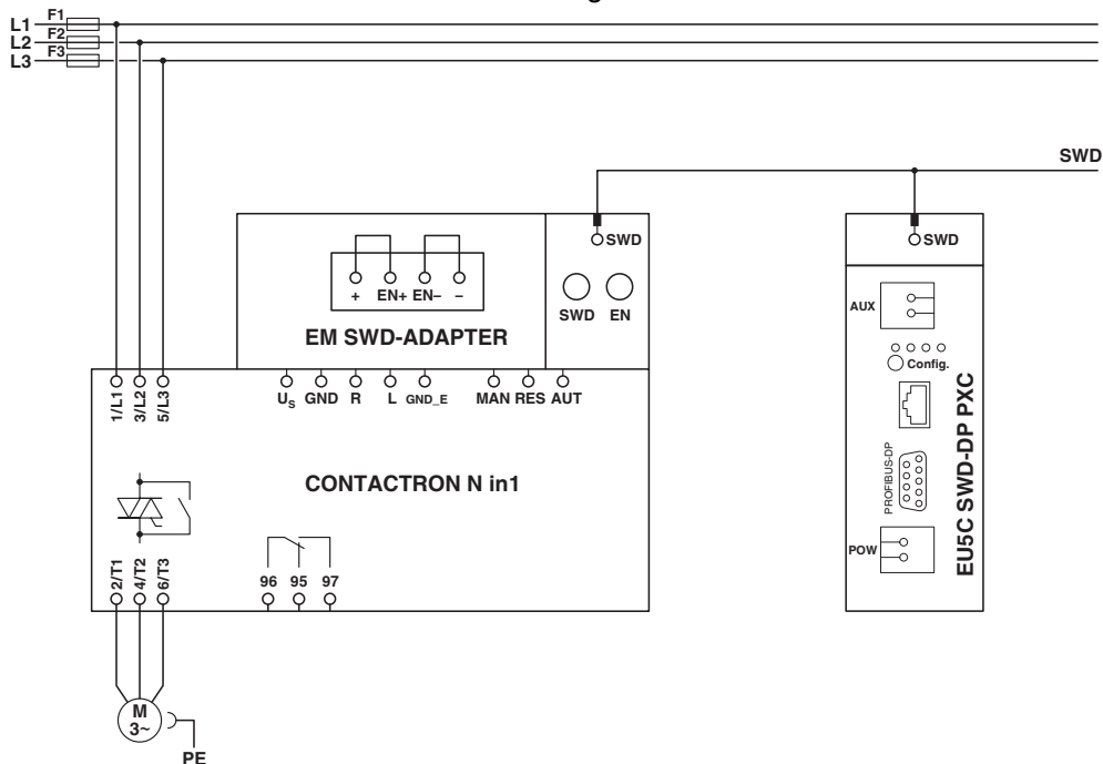
Circuit diagram
