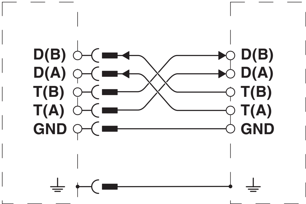
Connection diagram
