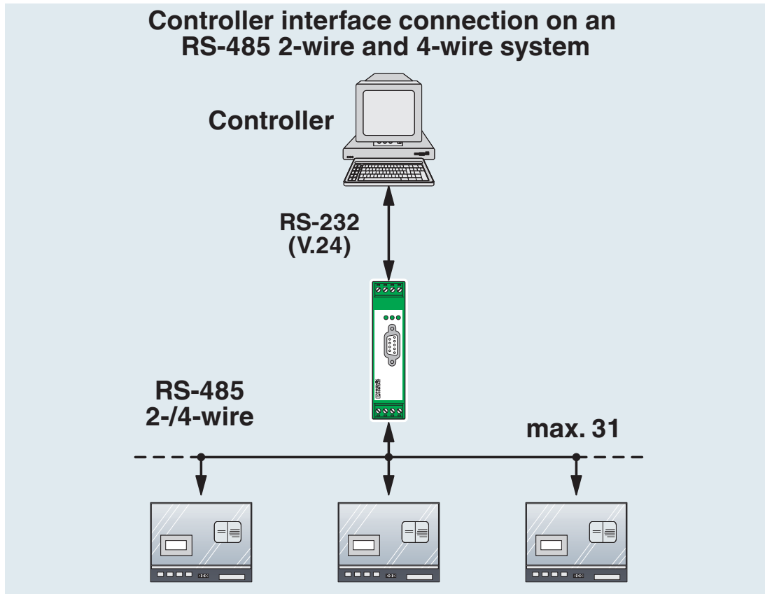
Application drawing
